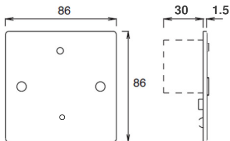
KSRA1 Face Plate with Light and Buzzer Alarm.
